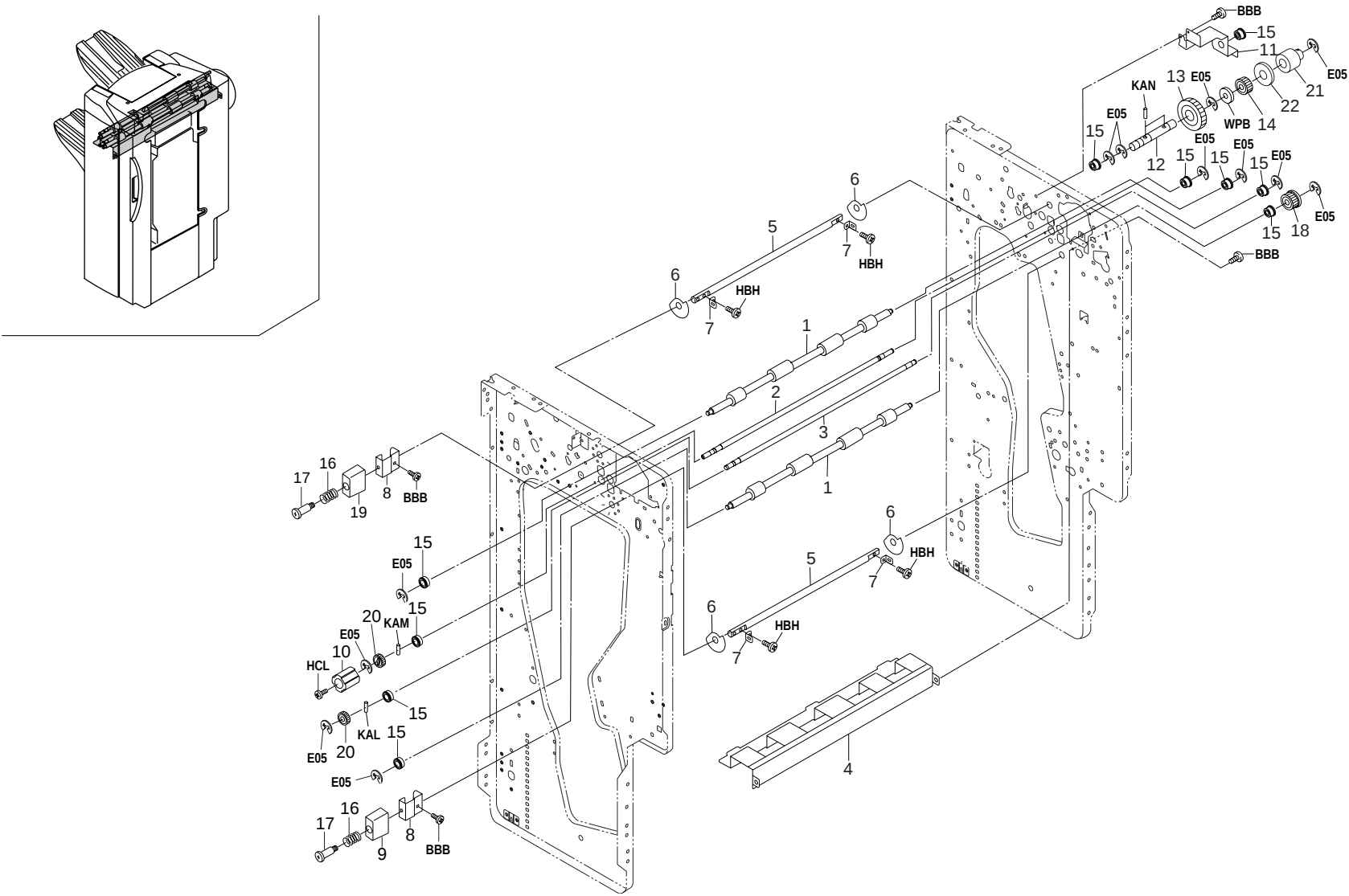
FIG. 12 DECURLER
