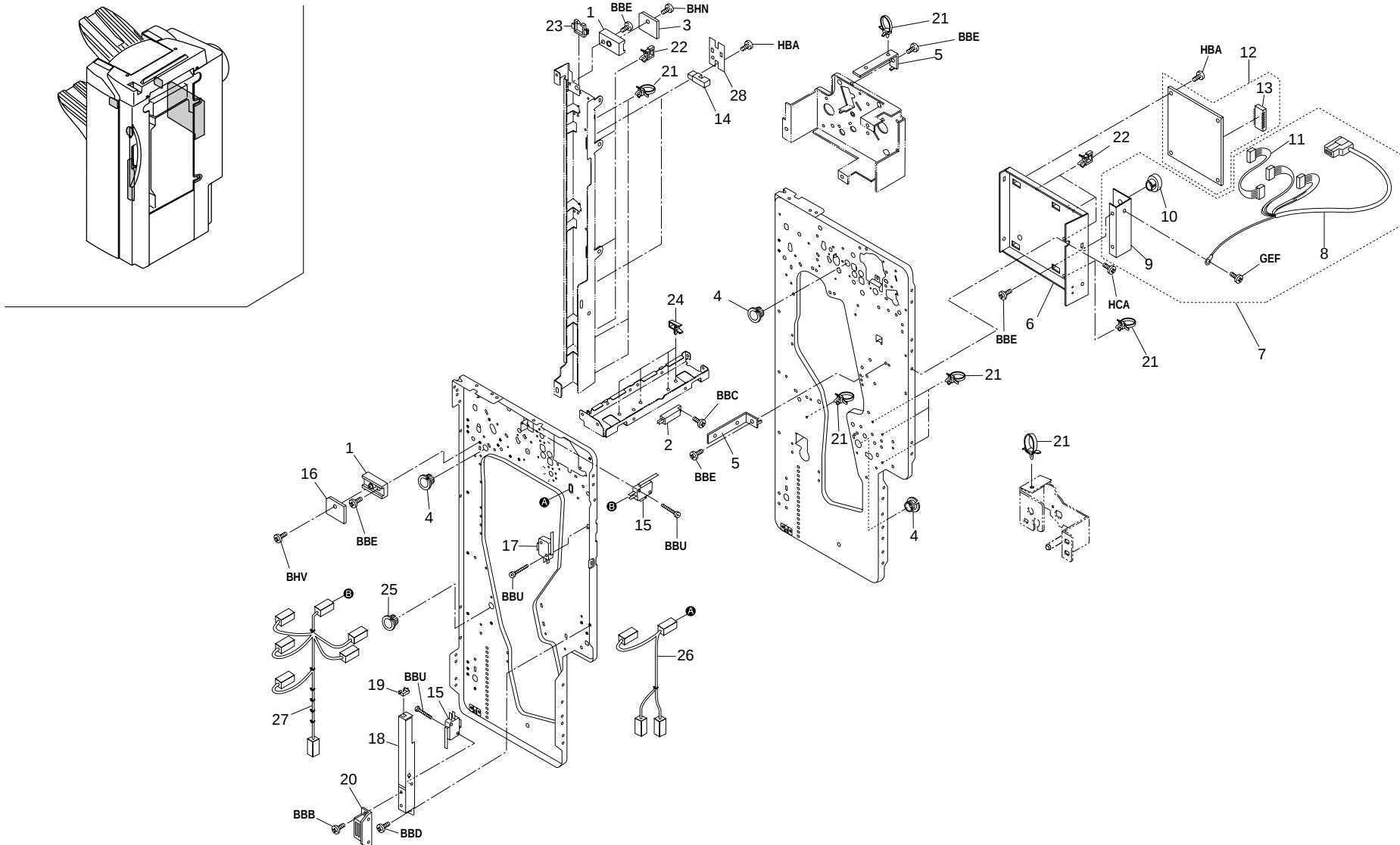
FIG. 10 ELECTRICAL COMPONENTS I
